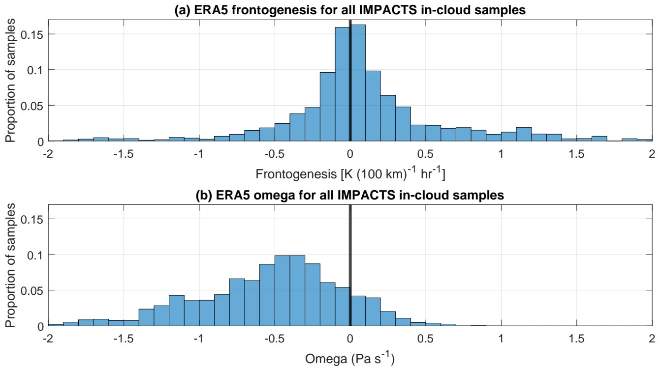
Figure 9. Distributions of ERA5 (a) frontogenesis [ \text{K (100 km)}^{-1} \text{hr}^{-1} ] and (b) omega ( \text{Pa s}^{-1} , where negative values indicate upward motion) for all IMPACTS P-3 in-cloud samples. For each IMPACTS sample point, the ERA5 frontogenesis and omega value at the nearest grid point at the nearest hour is taken. The 10th, 50th, and 90th percentiles of ERA5 frontogenesis for IMPACTS in-cloud sampled are -0.41 , 0.03 , and 0.79 \text{ K (100 km)}^{-1} \text{ h}^{-1} , respectively. For omega, the 10th, 50th, and 90th percentiles are -1.20 , -0.47 , and 0.05 \text{ Pa s}^{-1} , respectively.
