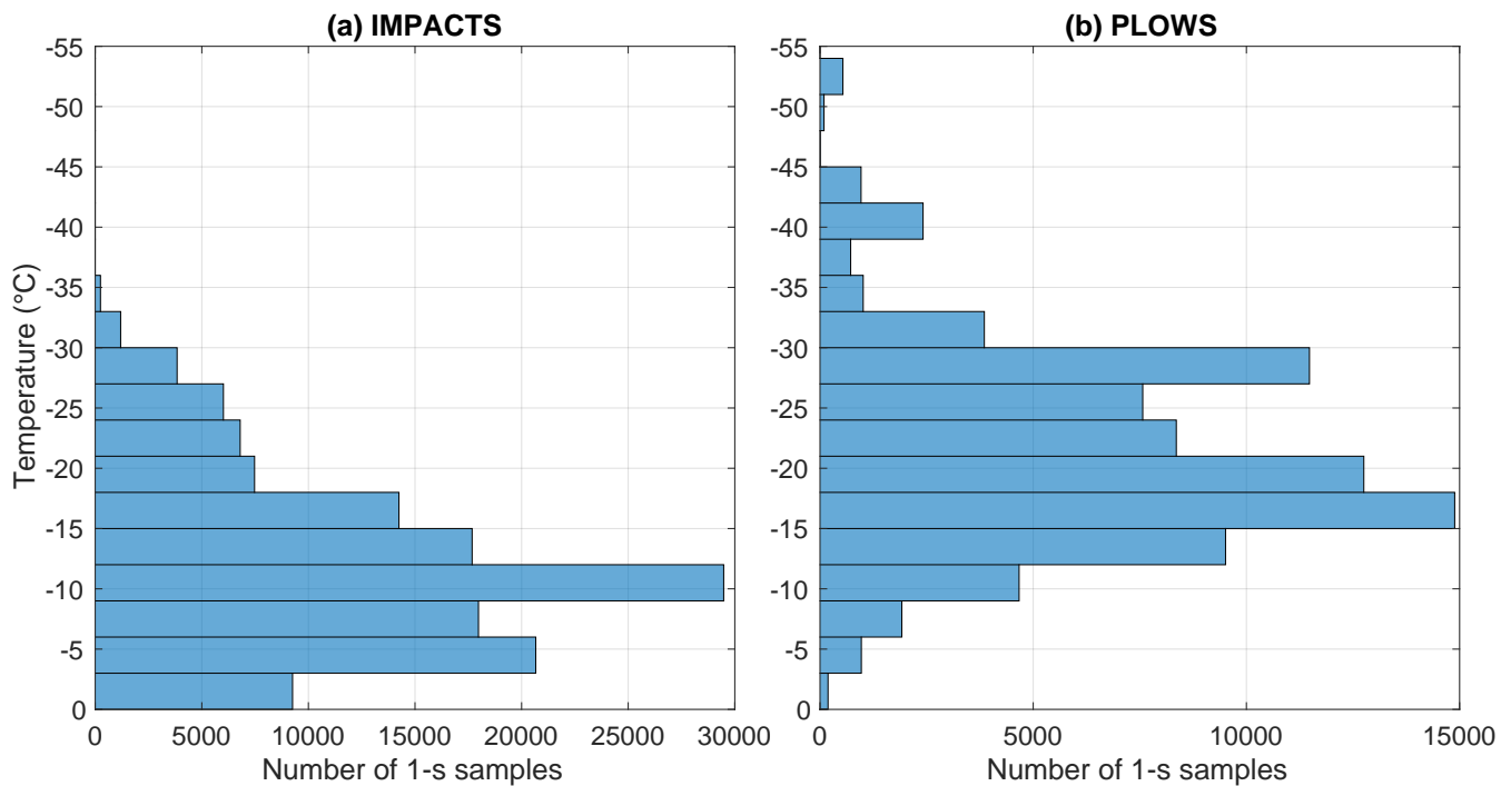
Figure 10. Distributions of in-cloud temperatures sampled during (a) IMPACTS and (b) PLOWS. Colder temperatures are at the top of each plot. The in-cloud environments sampled during PLOWS tended to be colder than those sampled during IMPACTS.
